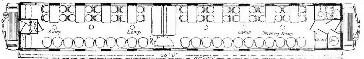
Fig. 162. CLUB CAR NETHERWOODS. CENTRAL RAILROAD OF NEW JERSEY.
